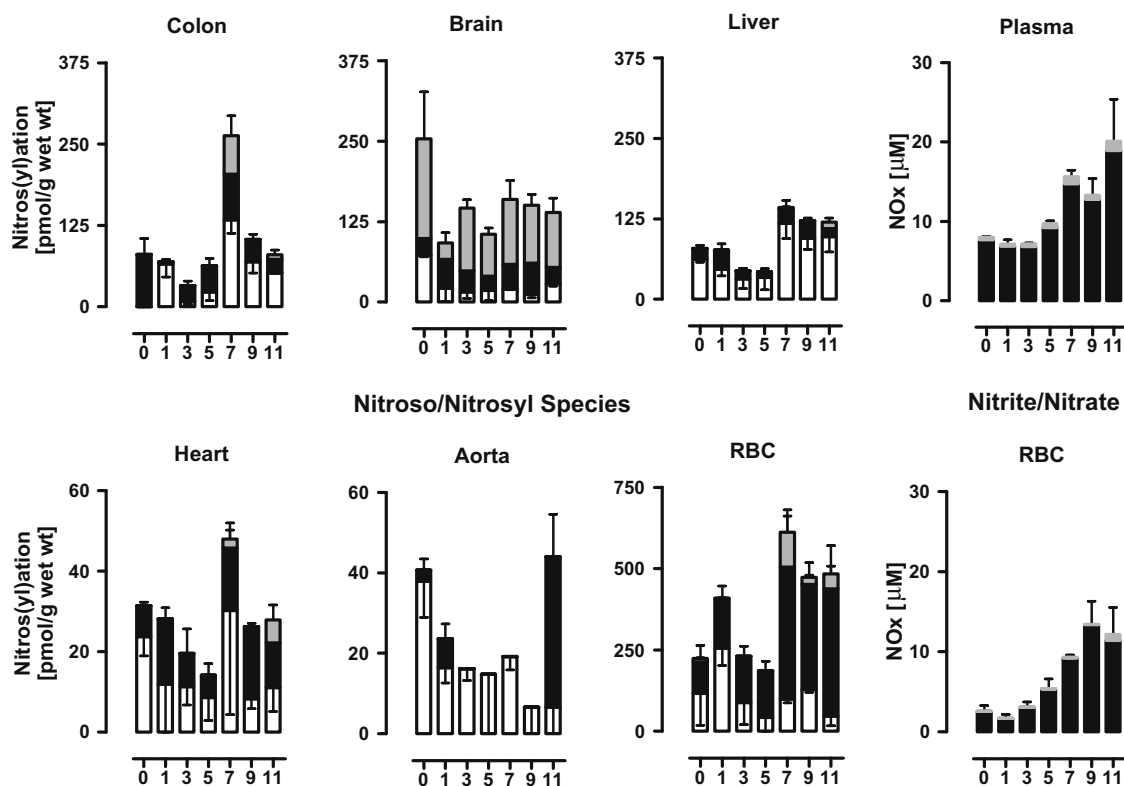
Fig. 2. Systemic changes in concentration of NO-related metabolites in blood and exemplary tissues of the rat during development of acute colon inflammation during DSS administration (days 0–7) and following cessation of DSS treatment (recovery phase; days 9–11). Nitrosyl(yl)ation products are exemplified by S-nitrosothiols (white), N-nitrosamines (black) and nitrosyl heme species (grey), whereas nitrate (black) and nitrite (grey) represent products of oxidative NO metabolism ( \text{NO}_x ). Data are means \pm SEM; n = 3/\text{day}/\text{tissue} .
