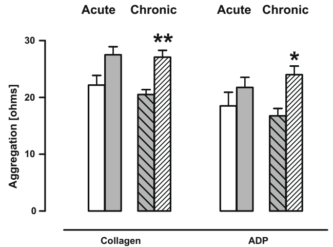
Fig. 6. Platelet aggregation as assessed by addition of collagen and adenosine diphosphate (ADP) to whole blood under control conditions (white bars, n = 6 ) and following 7 days of DSS administration (grey bars, n = 4 ) and in the chronic model of colon inflammation (white hatched bars, n = 9 ) with time-matched controls (grey lined bars, n = 4 ). Data displayed as means \pm SEM (* p < 0.05 , ** p < 0.01 versus control).
