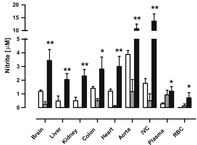
Fig. 4. Blood and tissue concentration of nitrite in controls (white bars, day 0), following 7 days DSS treatment (grey bars, day 7) and 4 days after treatment cessation (black bars, day 11). Data displayed as means \pm SEM, n = 3 /day/tissue. Where * represents p < 0.05 and ** represents p < 0.01 versus matched control (day 0). IVC, inferior vena cava; RBC, red blood cells.
