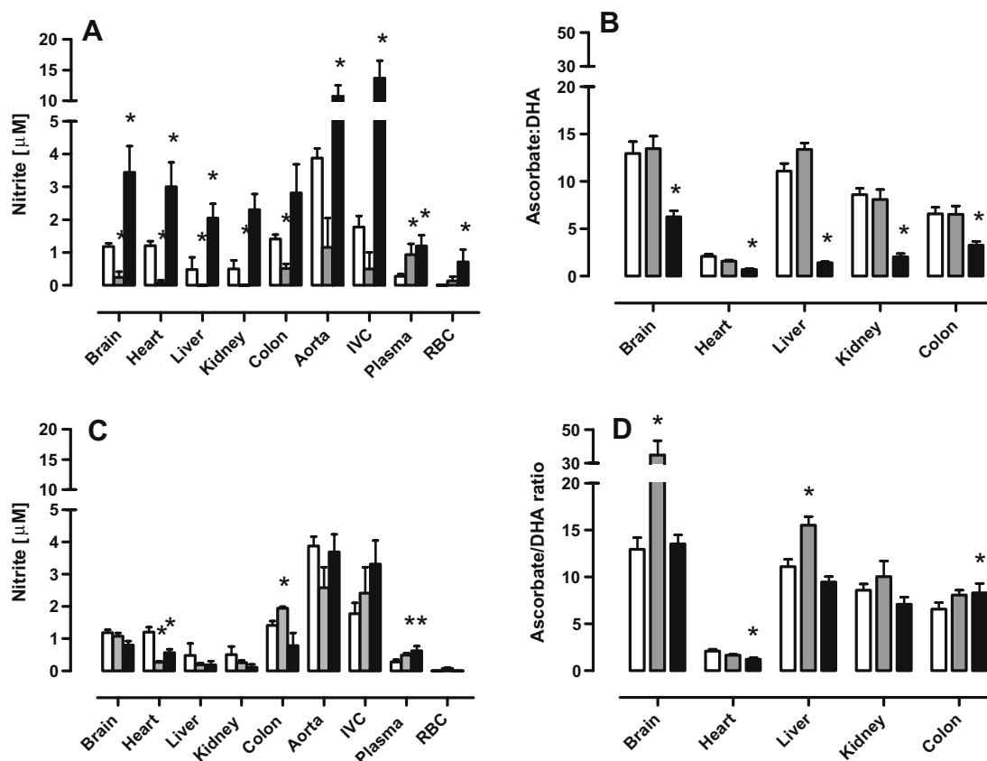
Fig. 8. Comparison of changes in nitrite concentration and ascorbate redox status in blood and tissues of DSS-treated animals in the absence (A and B) and presence (C and D) of 5-ASA. Upper panel: (A) Blood and tissue concentrations of nitrite and (B) tissue concentrations of ascorbate and dehydroascorbate (DHA; displayed as a ratio of ascorbate/DHA) in controls on day 0 (white bars), day 7 (grey bars) and day 11 (black bars). Lower panel: (C) Blood and tissue concentrations of nitrite and (D) tissue concentrations of ascorbate and dehydroascorbate (DHA; displayed as a ratio of ascorbate/DHA) on day 0 (white bars), day 7 (grey bars) and day 11 (black bars) of DSS administration with concomitant 5-ASA treatment starting on day 5. Data displayed as means \pm SEM from 3 animals/day ( *p < 0.05 ). IVC, inferior vena cava; RBC, red blood cells. No ascorbate/DHA measurements were performed in vascular tissue and blood due to limited sample availability.
