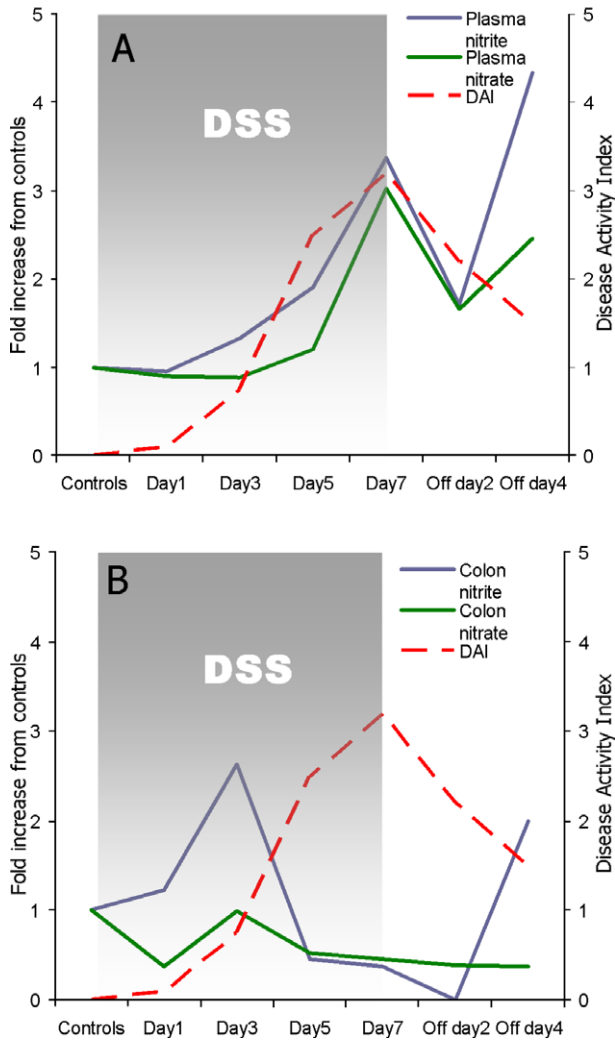
Fig. 3. Inflammatory response to continuous administration of DSS over a period of 7 days (area shaded in grey). The blue and green curves contrast the time course of nitrite and nitrate, respectively, with that of the DAI, in plasma (A) and in the colon (B). Each time point represents a fold-change from basal levels, calculated from the ratio of the mean concentration ( n = 3 ) at the day indicated on the X axis compared to the basal level ( n = 3 ) assessed at day 0 (Controls). Error bars were omitted for clarity.
