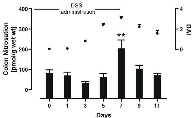
Fig. 1. Disease activity index (DAI) and concentration of total nitroso compounds in the colon of DSS-treated rats. Data displayed as mean \pm SEM, n = 3 /day. DAI was significantly increased from day 3 of DSS application on and remained significantly ( p < 0.01 ) elevated 4 days after cessation of DSS administration (asterisks omitted for sake of clarity). Colon nitrosation was significantly (** p < 0.01 ) increased on day 7 of DSS administration.
