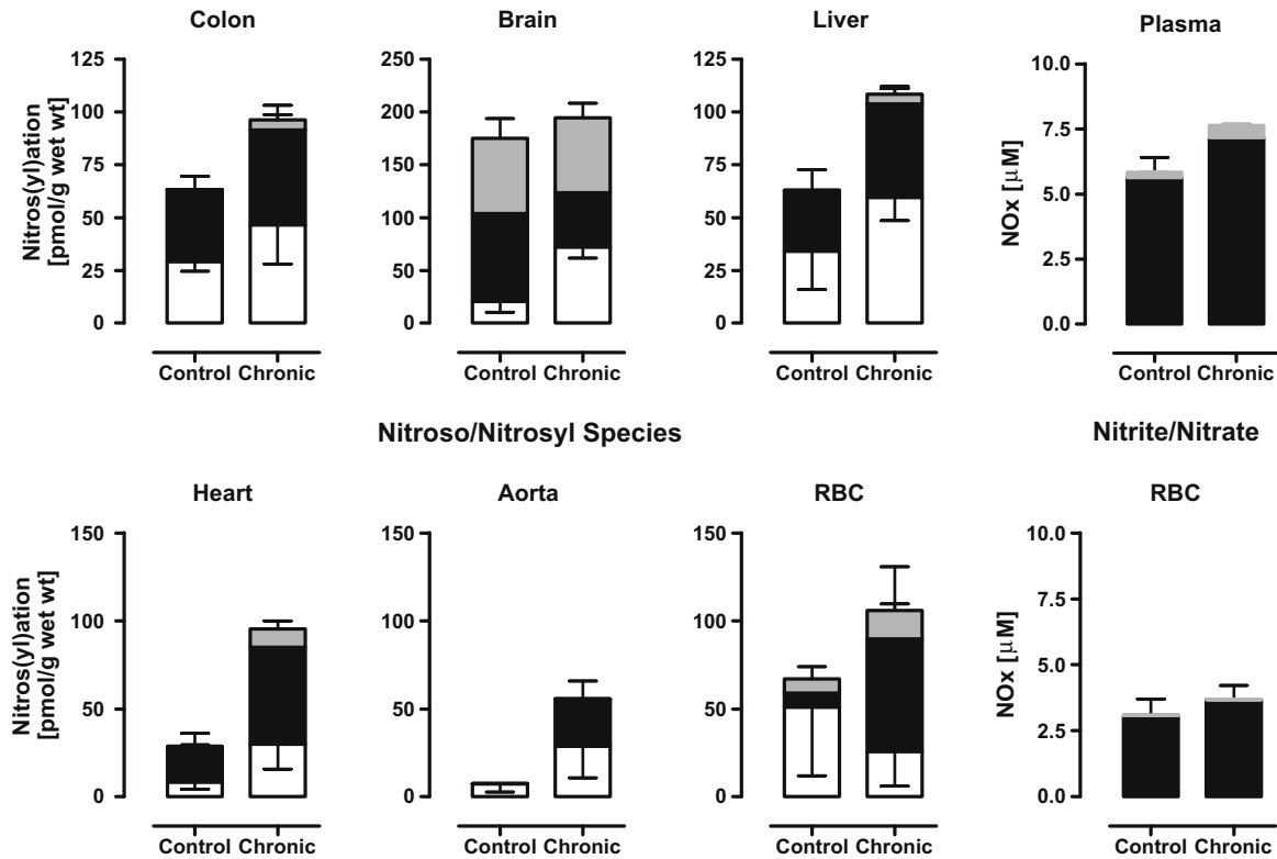
Fig. 7. Systemic changes in concentration of NO-related metabolites in blood and representative organs during chronic colon inflammation. Nitrosylation products are exemplified by S-nitrosothiols (white), N-nitrosamines (black) and nitrosyl heme species (grey), whereas nitrate (black) and nitrite (grey) represent products of oxidative NO metabolism ( \text{NO}_x ). Data are means \pm SEM, n = 5\text{--}6 /day/tissue.
