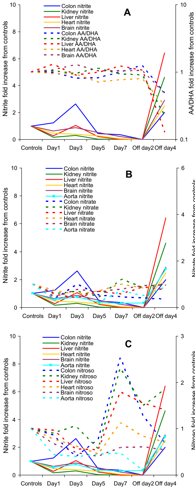
Fig. 5. Comparisons of the changes in redox status (expressed as AA/DHA ratio; A) as well as in the concentrations of nitrate (B) and nitroso products (C) with those in nitrite (solid curves) across various organs and in the circulation, in response to DSS administration over a course of 7 days followed by 4 days of recovery. Each time point represents a fold-change from basal levels, calculated from the ratio of the mean concentration ( n = 3 ) at the day indicated on the X axis compared to the basal level ( n = 3 ) assessed at day 0 (Controls). Error bars were omitted for clarity. Aortic AA/DHA levels were not determined due to limited sample size.
